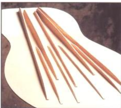
D: Ovation developed the Quintad bracing pattern to give the Elite tremendous power and projection.
